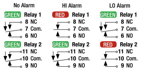
API 1420 G Alarm States with Normal Action HI/LO Alarms
