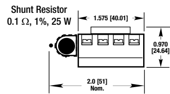
API 6010 G 5A 8-Pin Socket with Shunt, 600 V Rating
