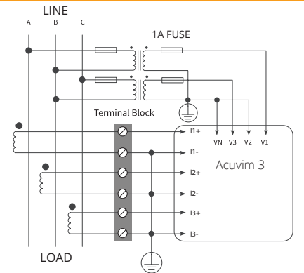
2 Element 3 Wire Delta - 3CT
