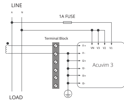
1 Element 2 Wire
